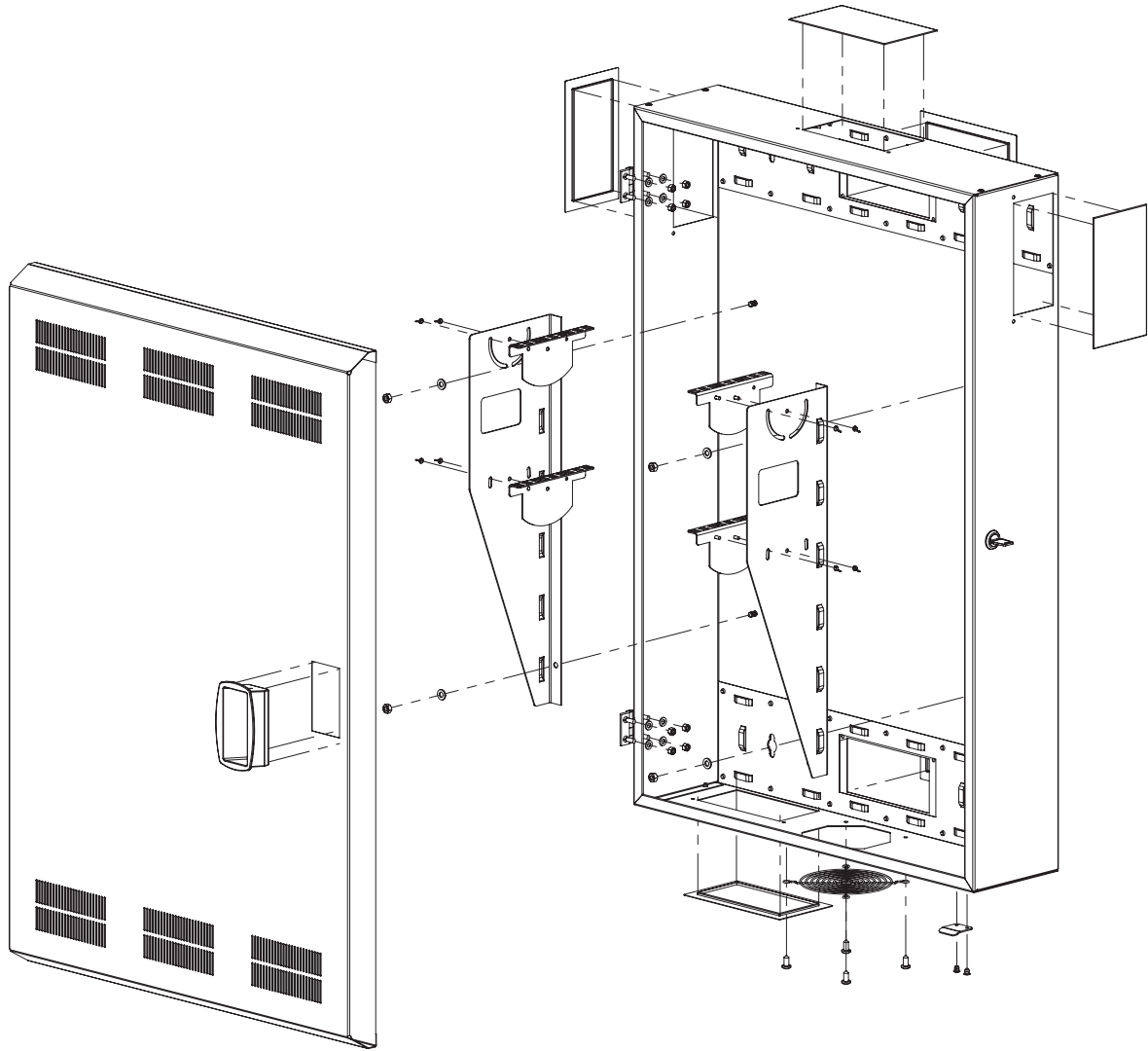
EXPLODED VIEW
