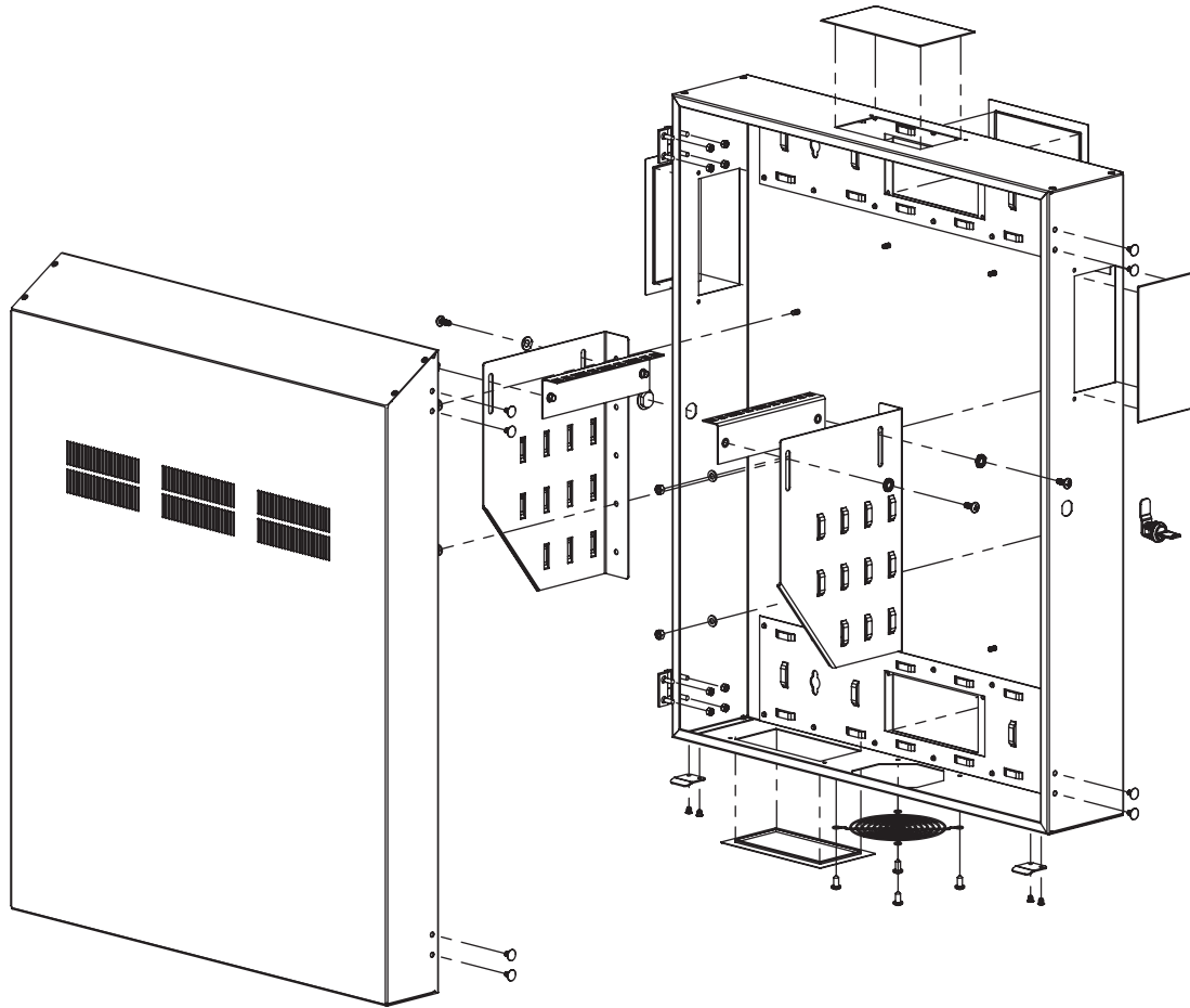
EXPLODED VIEW
