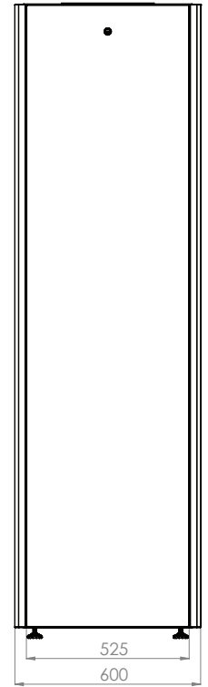
REAR VIEW
