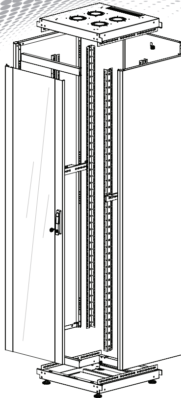
EXPLODED VIEW
