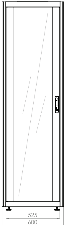
FRONT VIEW
