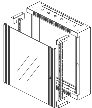
EXPLODED VIEW
