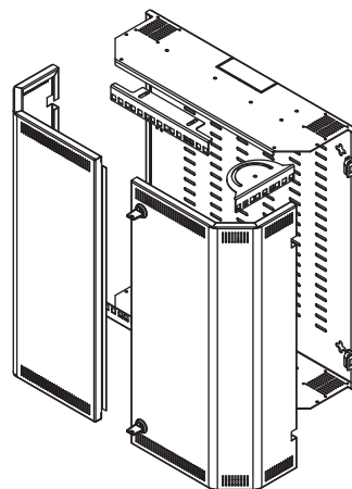
EXPLODED VIEW
