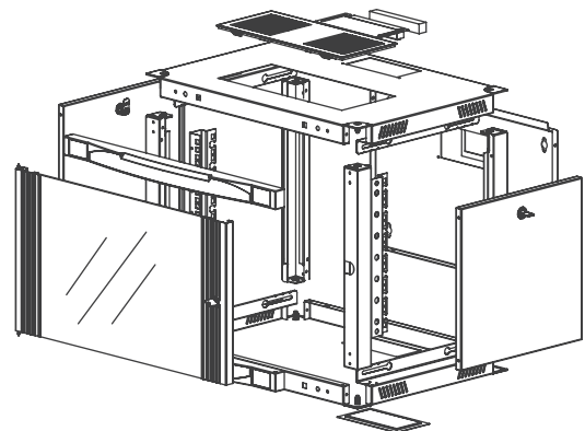
EXPLODED VIEW
