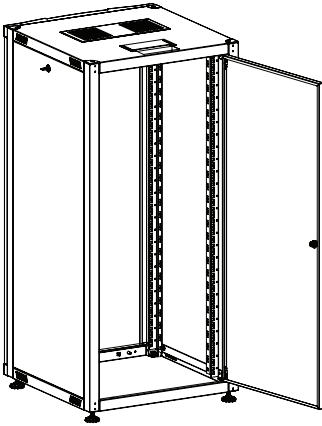
ISOMETRIC REAR VIEW WITH LEVELING FEET WITH HINGED REAR DOOR
