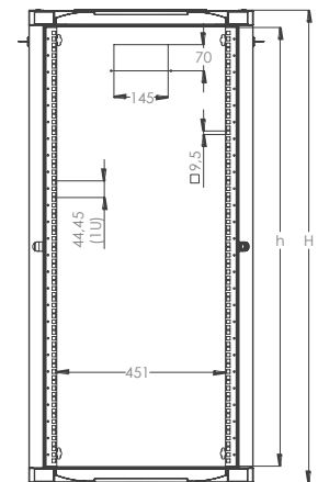
DIMENSIONS IN WIDTH AND HEIGHT
